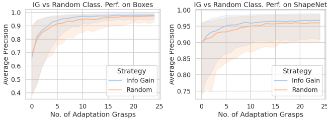
Fig. 6: Information Gain GNP encoders can be exploited for faster information-gathering. Average Precision per grasp for IG and random adaptation strategies. Solid lines are medians, and error ranges are the upper and lower quartiles across 500 test objects.
