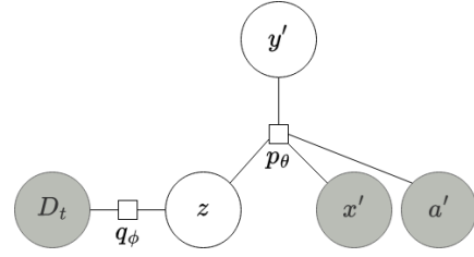
Fig. 2: After executing t actions and observing their outcomes, D_t , the robot can predict a posterior over the unobserved properties, q_\phi(z | D_t) . We aim to predict feasibility y' of unlabeled actions, a' , given an object's observed properties, x' , and current belief, z .
