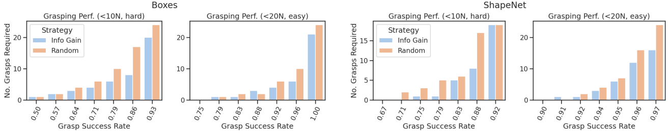
Fig. 7: GNP Performance as a Grasp Detector Number of adaptation grasps needed to reach a desired Grasp Success Rate . The GNP chooses the most likely grasp considering the current uncertainty arising from limited data. We consider easy and hard versions of the task that use different force limits. The IG adaptation strategy tends to produce higher success rates with fewer adaptation grasps.
