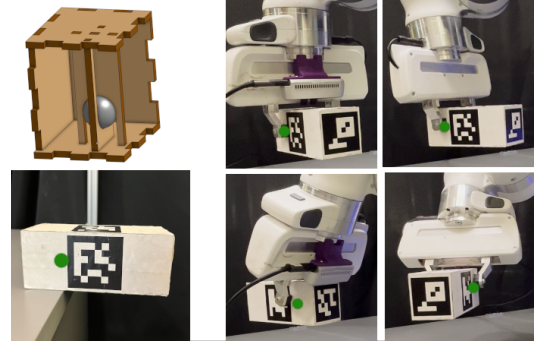
Fig. 9: Robot Demo We test our method on a Panda robot by grasping a block with an offset CoM (left). After 10 adaptation grasps, the robot consistently grasps the object near the CoM (green dot). The right 4 grasps show 4 successful evaluation grasps.
