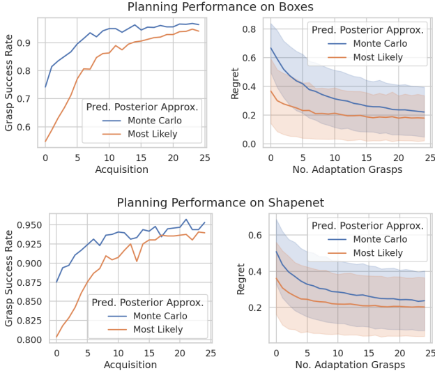
Fig. 8: Planning Success and Normalized Regret for the minimum force grasping task . We ablate our GNP model to show the impact of the explicit uncertainty representation. Solid lines are means and shaded regions are a standard deviation.
