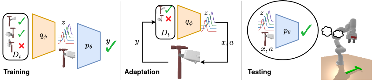
Fig. 3: Grasp Neural Processes use an offline training phase (left) to jointly learn an action feasibility model, p_\theta , and an inference network, q_\phi , that predicts a posterior distribution over unobserved properties. During the adaptation phase (center), the learned inference network can be used for efficient online posterior updates and action selection. Finally, in the testing phase (right), the robot can use the current belief, z , along with the feasibility model to perform manipulation tasks.
